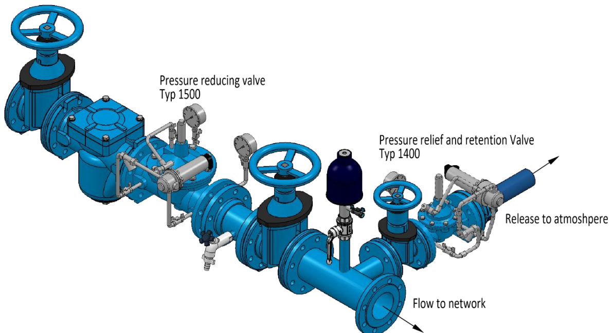
Type 1400, installation as a pressure relief valve
